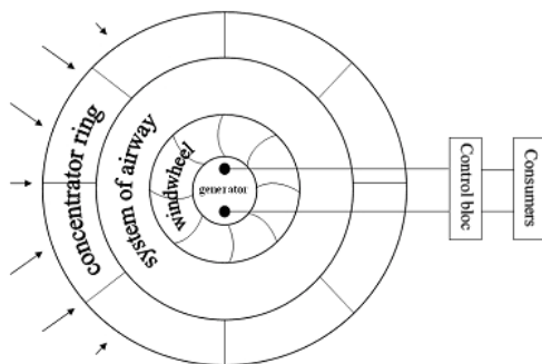
Fig.1. LSWT general block diagram
