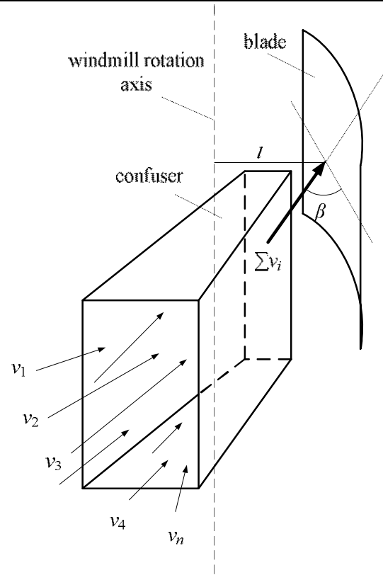
Fig. 6. Run an air stream on the blade
