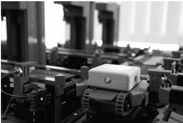
Fig. 2. Production system model
