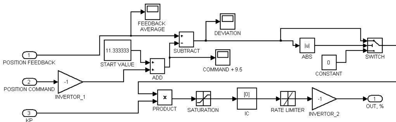
Fig. 3. Block “P-regulator of position” of the model RTC-1
