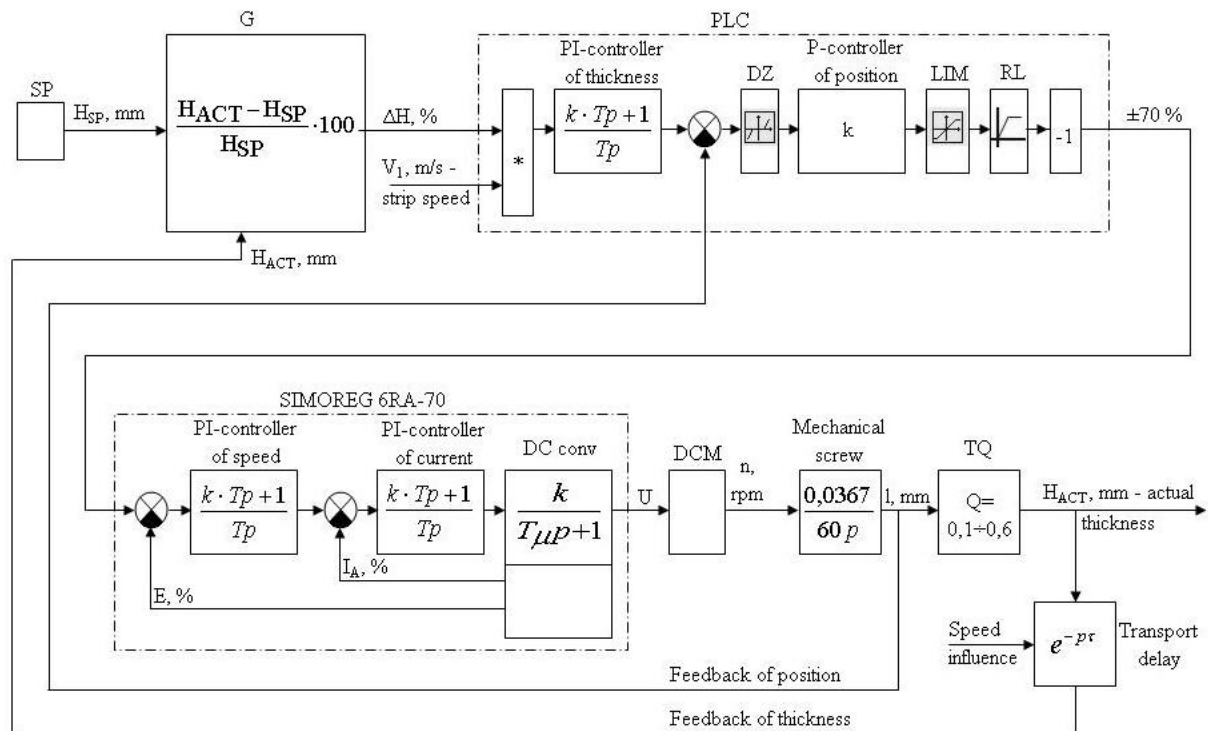
Fig. 1. Block diagram of the existing RTC-1 system
