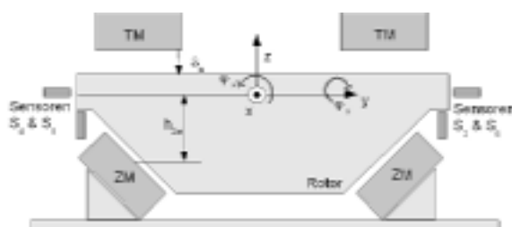
Fig.4. Side view of the magnetic levitation system
