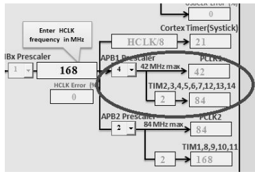
Fig.5 –Timer TIM4 clock frequency
