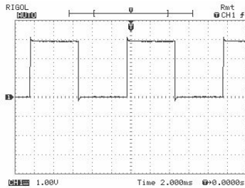
Fig.8 – PWM output signal waveform (D = 50 %)
