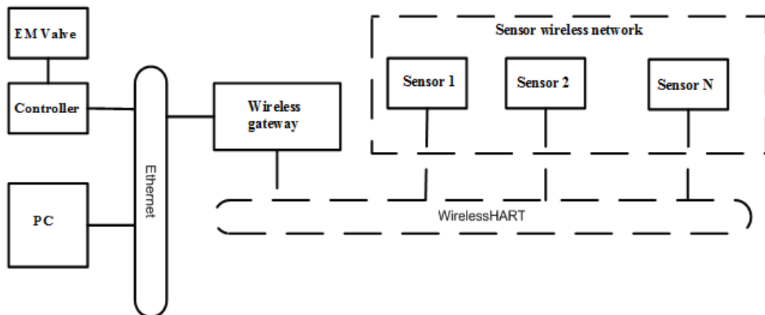
Fig. 3. Block diagram of the automatic control system for hydraulic soil washout
