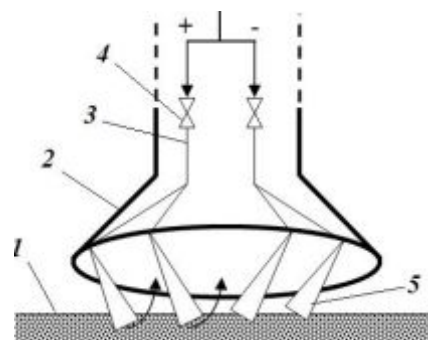
Fig. 1. The scheme of the hydraulic soil washout impulse system: 1 – soil; 2 – slurry intake unit; 3 – line for shock pressure waves discharge to the nozzle tip; 4 – control valves; 5 – shock pressure waves
